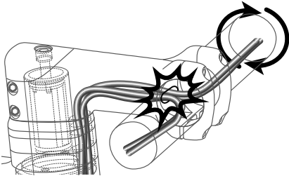
Fig. 1/26 Internally routed brake lines and shift cables
