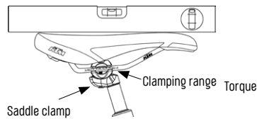
Fig. 4/25 Saddle assembly
