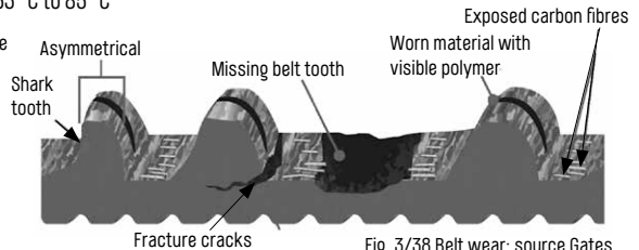
Fig. 3/38 Belt wear; source Gates
