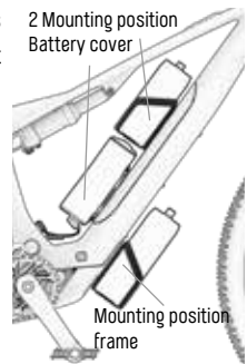
Fig. 1/52 Examples of mounting positions for EPACs
